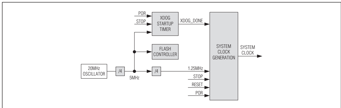
Figure 4. Clock Sources
